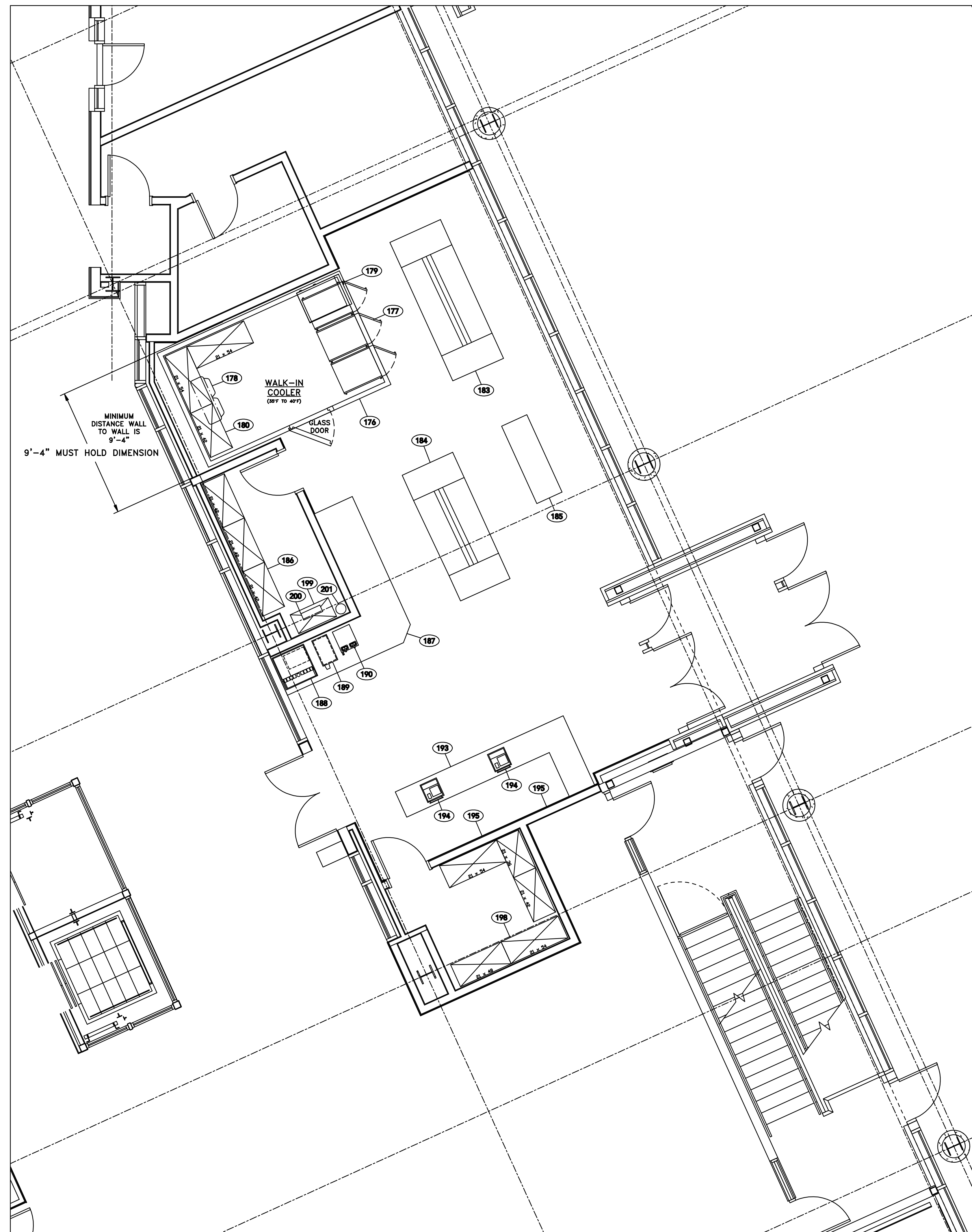
1 LEVEL 01 CONVENIENCE STORE EQUIPMENT PLAN Scale: 1/4"=1'-0"
