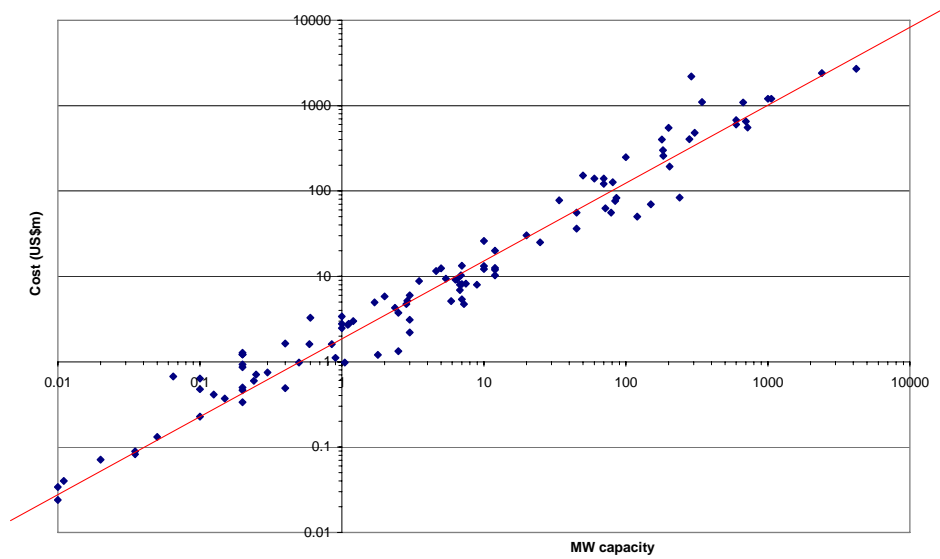
Figure 5 – Relationship between plant cost and capacity.
